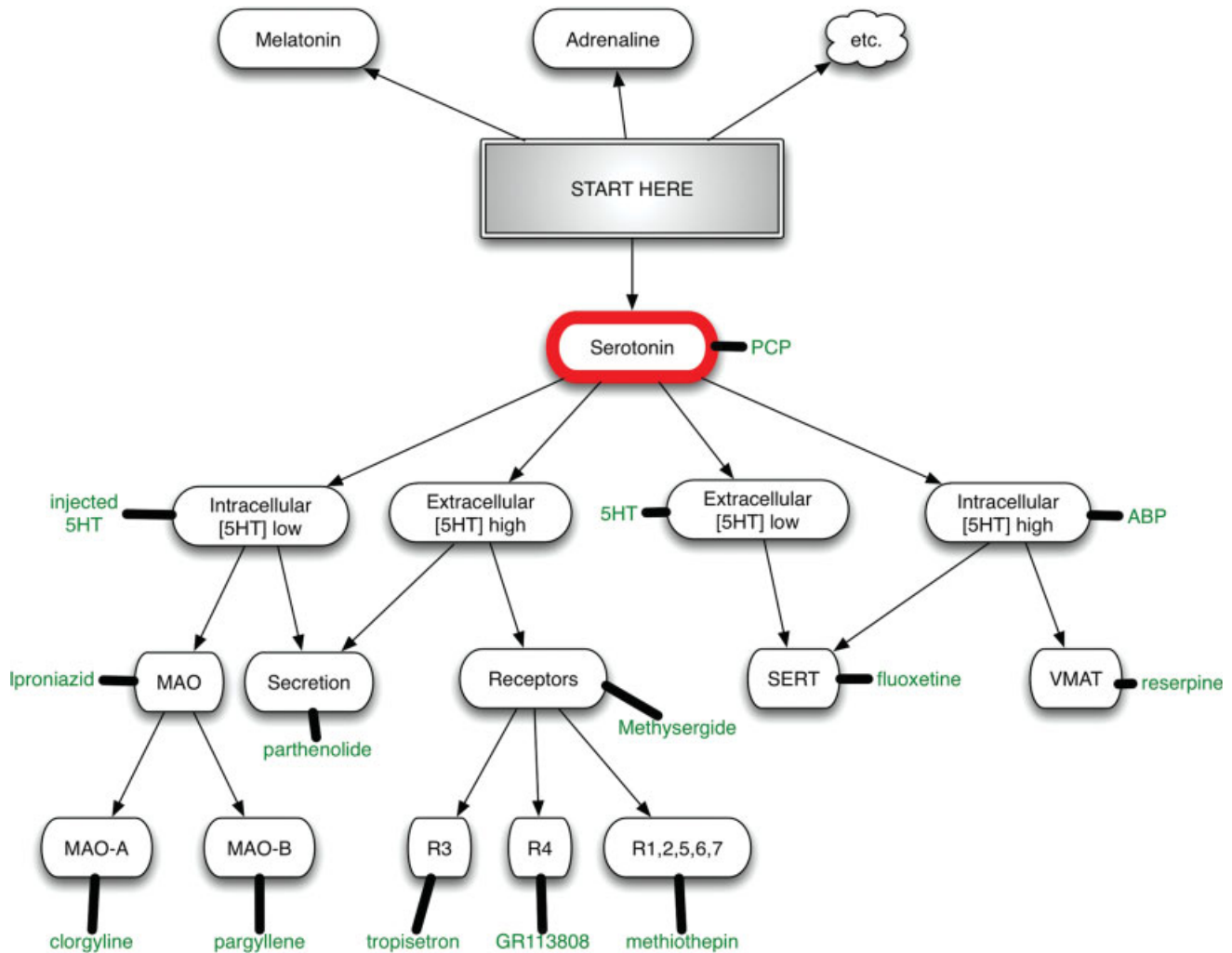
FIG. 3. A more complex strategy for probing neurotransmitter effects in a POI. Oval nodes represent specific functional modules (proteins or physiological conditions) whose involvement is to be tested. For reasons of space, lower tiers have been left out of this diagram. For example, the serotonin receptor 1 family is subdivided into types 1a, 1b, 1d, 1e, 1f, 1p, and 1s. Green labels indicate an example of reagents that can be used to test the node to which they are attached. Arrows between two nodes indicate suggested screen paths to be taken depending on the outcome of each result. [Color figure can be viewed in the online issue, which is available at www.interscience.wiley.com .]
