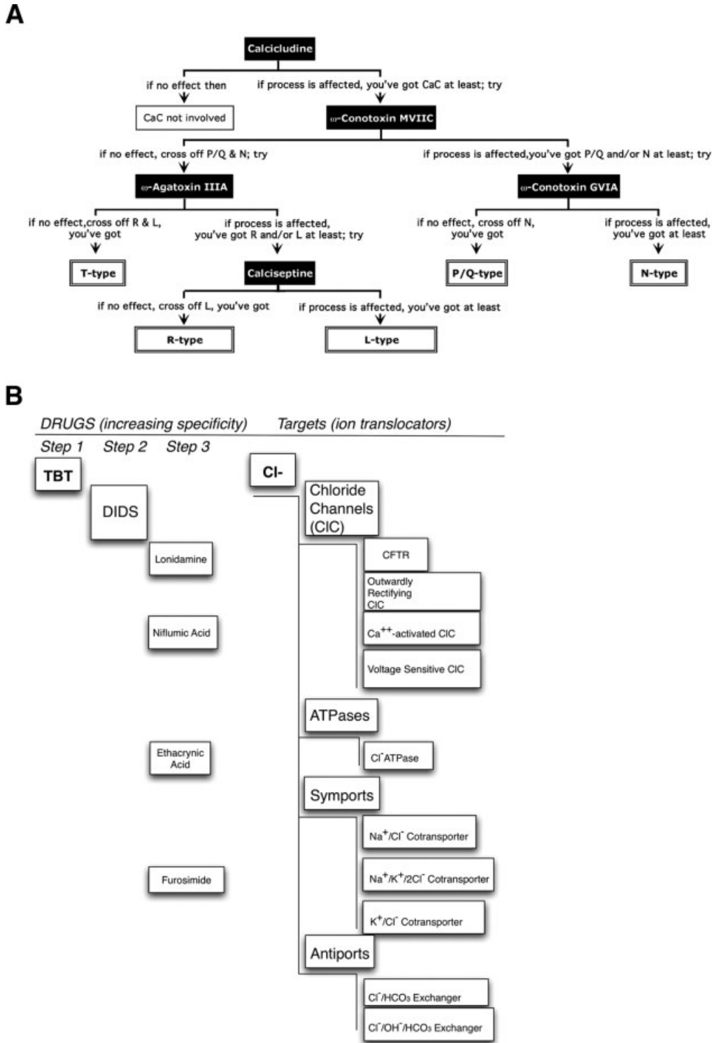
FIG. 2. Sample decision trees for testing the involvement of calcium (A) and chloride (B) signaling in a POI. Panel (a) illustrates the detailed logic for traversing a data tree to identify a calcium conductance. Panel (b) simply illustrates the corresponding drug and transporter trees for chloride.
